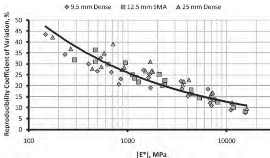
Figure 26. Final dynamic modulus reproducibility coefficient of variation.
