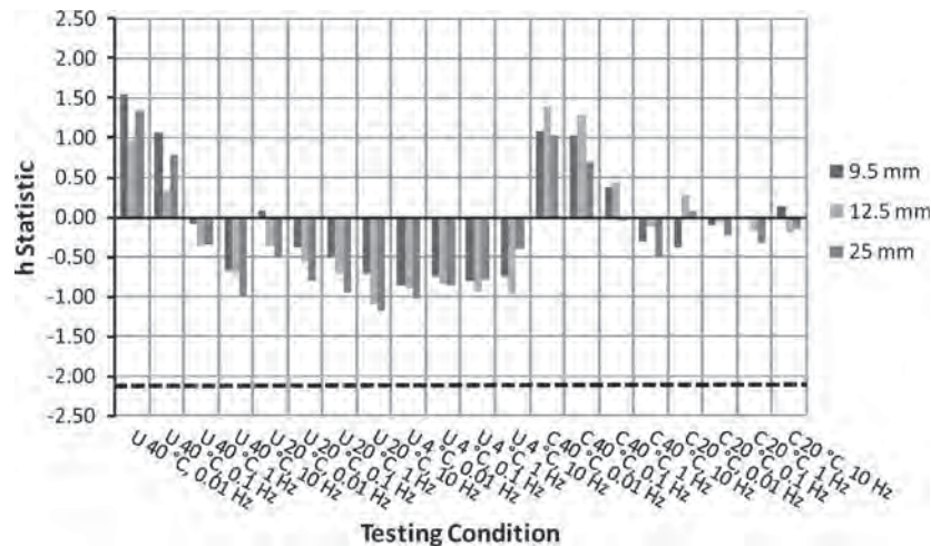
Figure D2. Between-laboratory dynamic modulus consistency statistic, h , for Lab 1.
