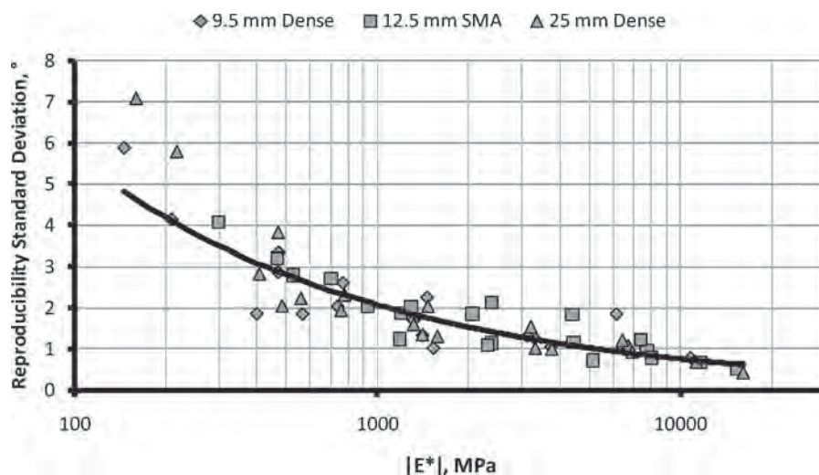
Figure 16. Prefabricated core phase angle repeatability standard deviation.
