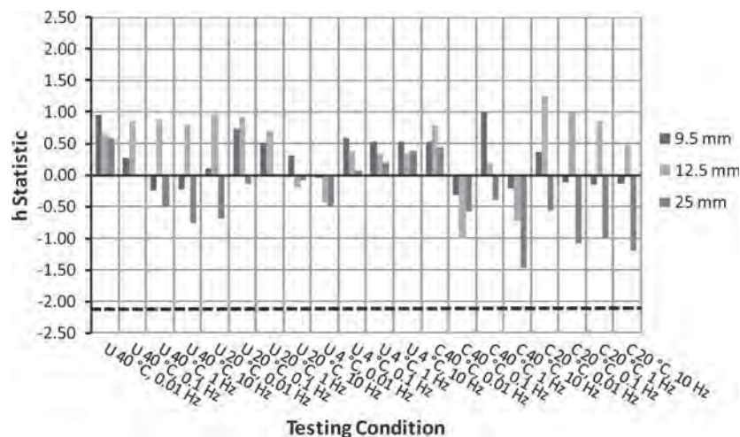
Figure E16. Between-laboratory dynamic modulus consistency statistic, h , for Lab 8.
