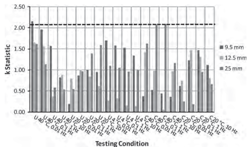
Figure D27. Within-laboratory phase angle consistency statistic, k , for Lab 6.
