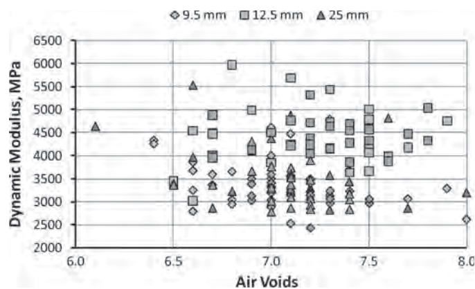
Figure 45. Effect of air voids on unconfined dynamic modulus for 20°C and 1.0 Hz loading.
