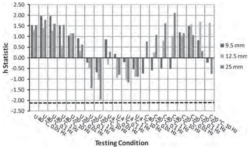
Figure E24. Between-laboratory phase angle consistency statistic, h , for Lab 4.
