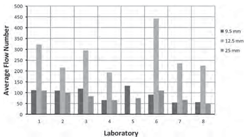
Figure 31. Average flow number for prefabricated cores.
