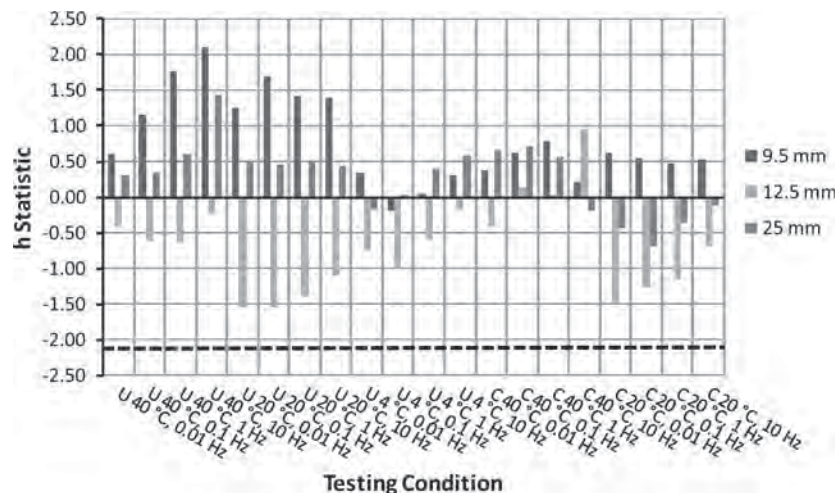
Figure E6. Between-laboratory dynamic modulus consistency statistic, h , for Lab 3.
