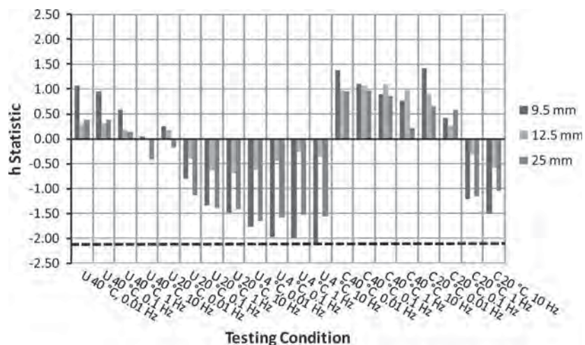
Figure D28. Between-laboratory phase angle consistency statistic, h , for Lab 6.
