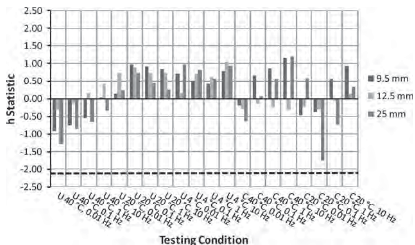
Figure D26. Between-laboratory phase angle consistency statistic, h , for Lab 5.
