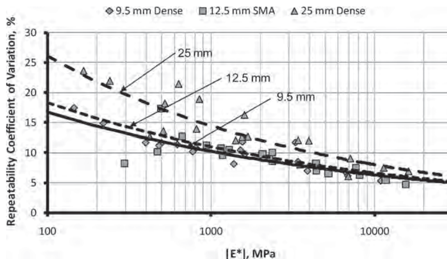
Figure 24. Final dynamic modulus repeatability coefficient of variation.
