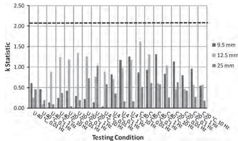
Figure E21. Within-laboratory phase angle consistency statistic, k , for Lab 3.
