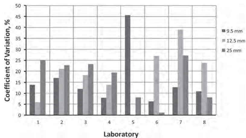
Figure 32. Variability of flow number for prefabricated cores.
