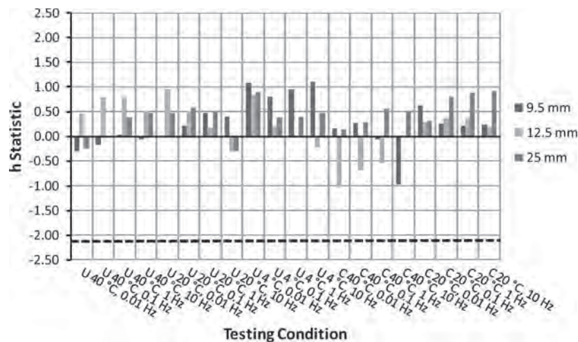
Figure E12. Between-laboratory dynamic modulus consistency statistic, h , for Lab 6.
