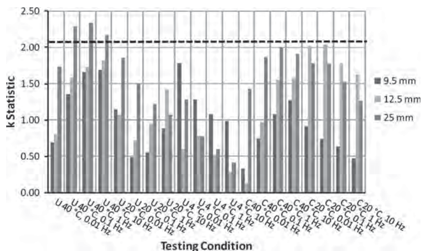
Figure D5. Within-laboratory dynamic modulus consistency statistic, k , for Lab 3.
