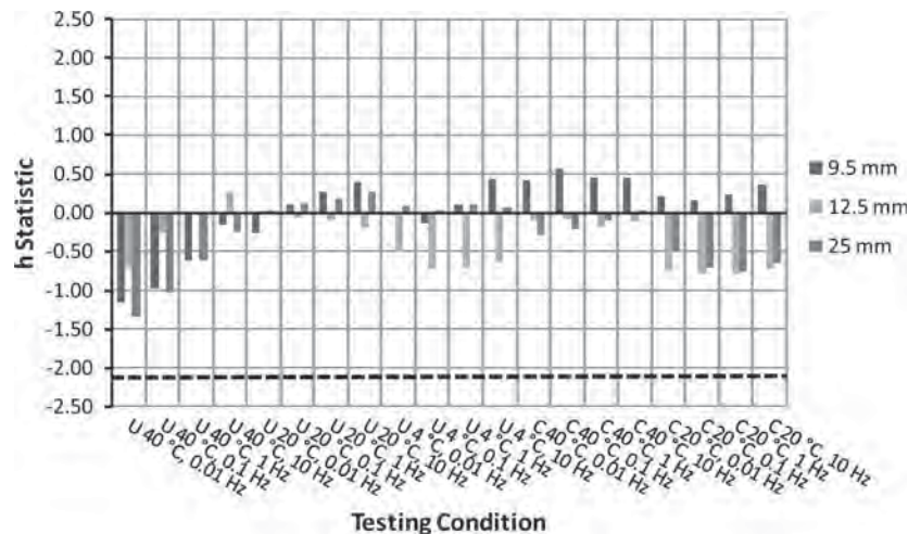
Figure D14. Between-laboratory dynamic modulus consistency statistic, h , for Lab 7.
