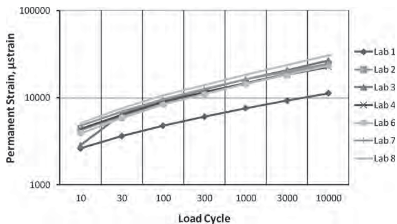
Figure 39. Average permanent strain from confined flow number tests on prefabricated cores.
