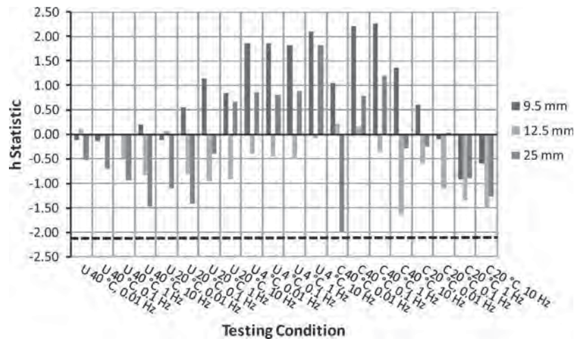
Figure E26. Between-laboratory phase angle consistency statistic, h , for Lab 5.
