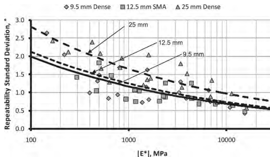
Figure 25. Final phase angle repeatability standard deviation.
