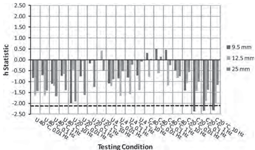
Figure E14. Between-laboratory dynamic modulus consistency statistic, h , for Lab 7.
