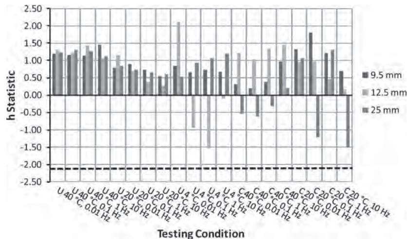
Figure D24. Between-laboratory phase angle consistency statistic, h , for Lab 4.
